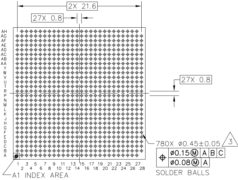
BOTTOM VIEW
