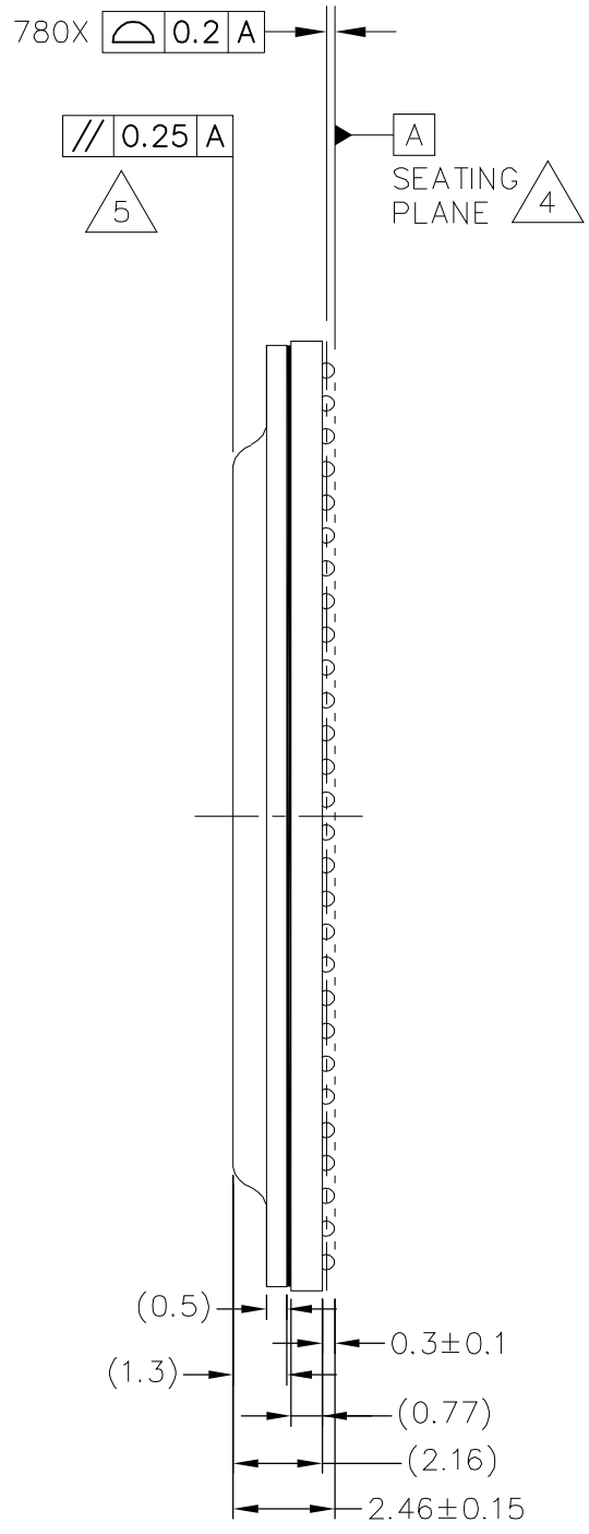
VIEW D-D
